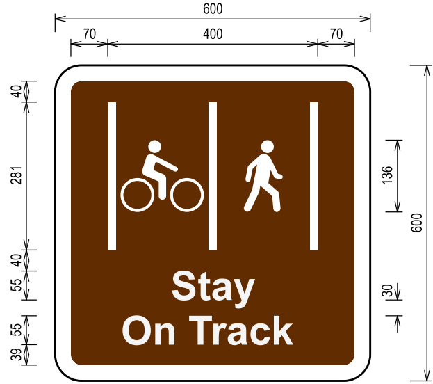
STAY ON TRACK THESE SIGNS ARE USED TO INDICATE A SEGREGATED TRACK. USUALLY PLACED AT THE START OF THE TRACK.
