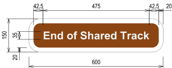
END OF SHARED TRACK THIS SIGN IS USED TO INDICATE THE END OF SHARED TRACK. USUALLY PLACED AT THE END OF THE TRACK.
