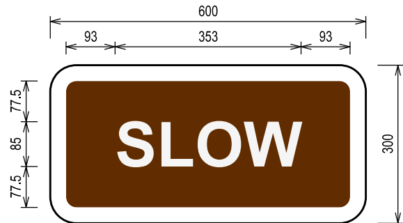
SLOW (SUPPLEMENTARY) TO BE PLACED BELOW STANDARD SIGNAGE, WHERE NECESSARY.
