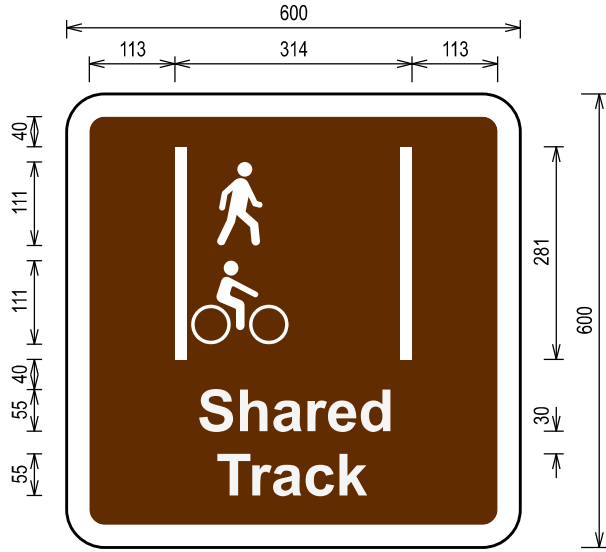
SHARED TRACK THIS SIGN IS USED TO INDICATE A SHARED TRACK. USUALLY PLACED AT THE START OF THE TRACK.
