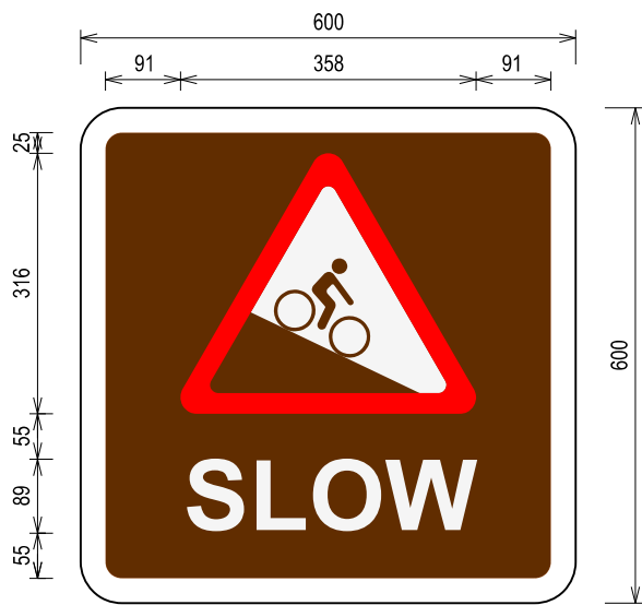
SLOPE AHEAD THIS SIGN INFORMS CYCLISTS THERE IS SLOPE AHEAD AND TO SLOW THEIR SPEED
